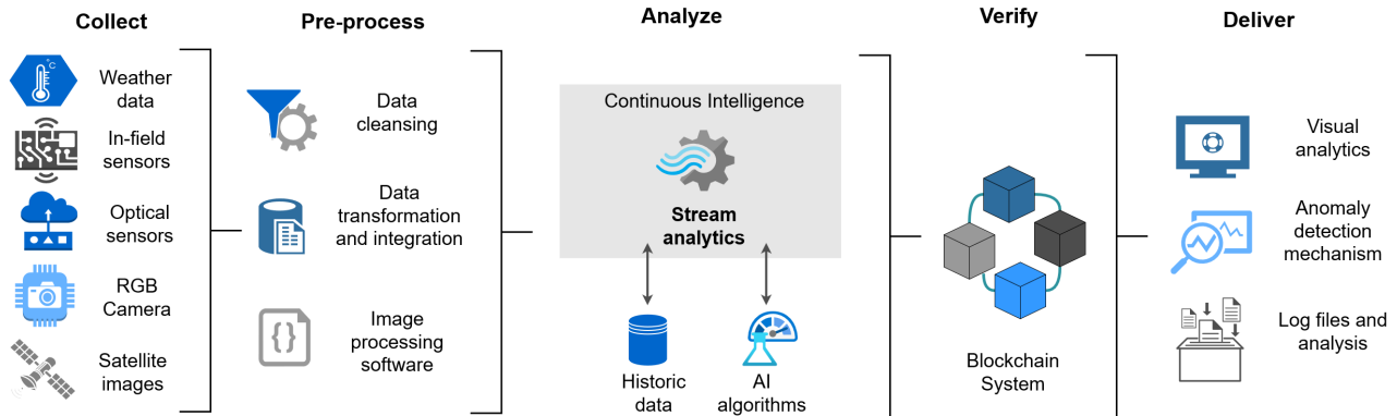
Fig. 1. PestNu data stream conceptual architecture
