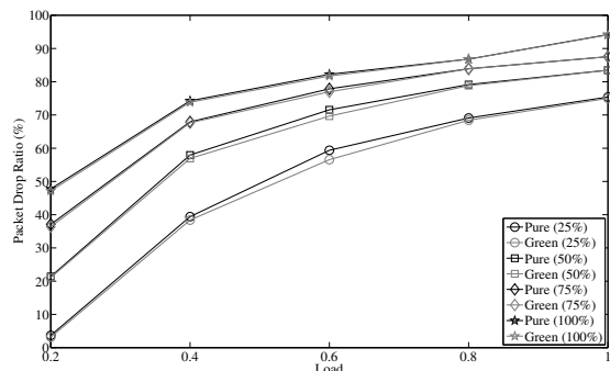
Figure 7. Packet drop ratio (two data channels).
