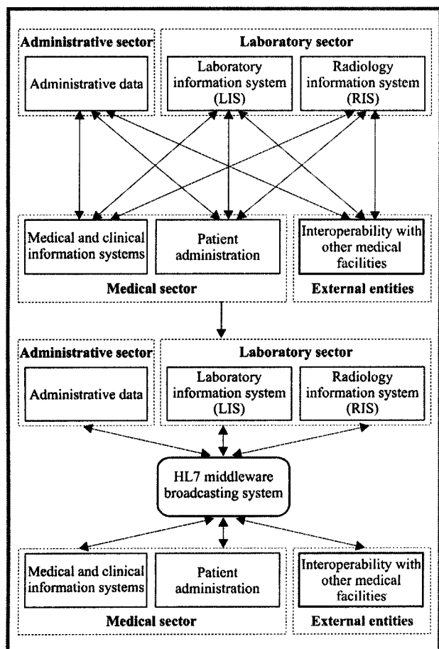
Fig. 4. Creating an interoperability framework.
