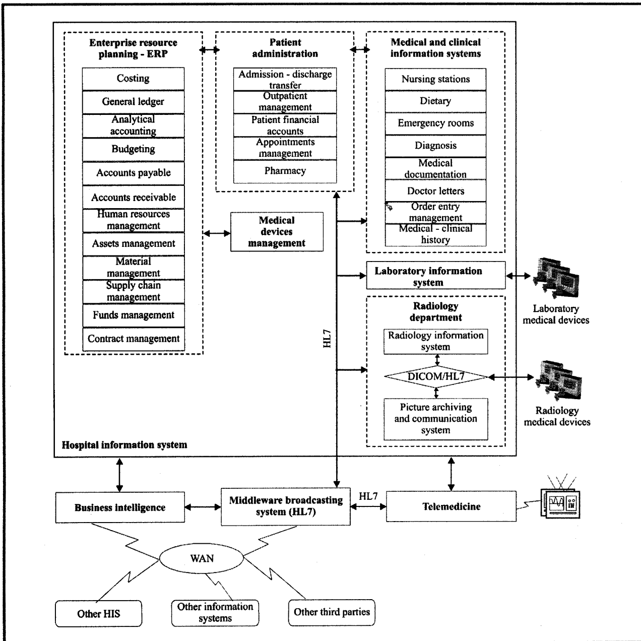
Fig. 1. Regional healthcare information system basic software components.
