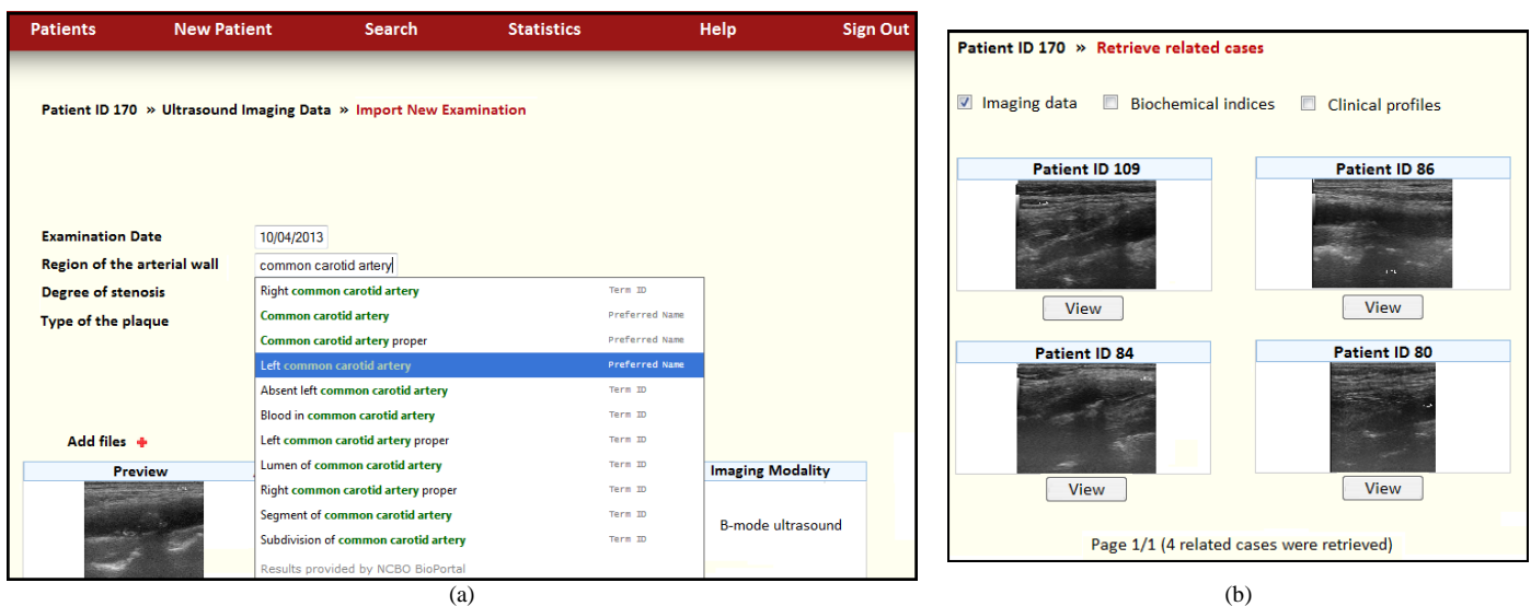
Fig. 6. Snapshots of CAROTID usage at the stage of (a) importing ultrasound imaging data for a new patient, completing the examination date, degree of stenosis, and type of the plaque [39], and annotating the position of the atherosclerotic plaque using FMA ontology, and (b) retrieving imaging data for similar stored cases.
